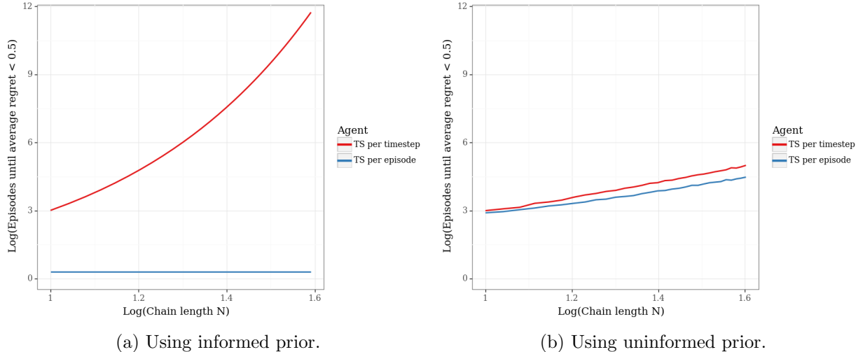
Figure 19: Comparing Thompson sampling by episode with Thompson sampling by timestep.
