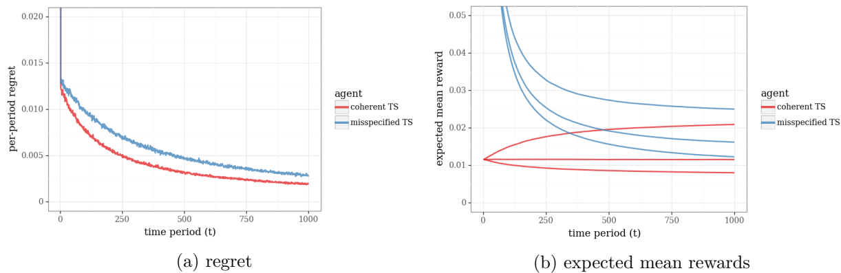
Figure 11: Comparison of Thompson sampling for the Bernoulli bandit problem with coherent versus misspecified priors.
