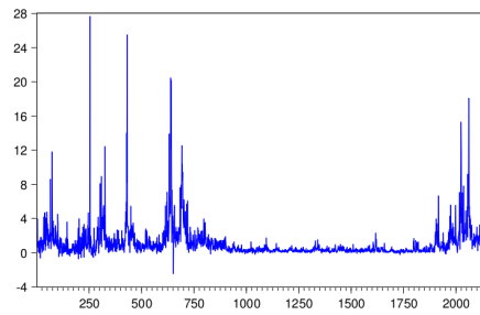
Figure 18: Line Graph of daily RC computed from 5-min returns of IBM and Citigroup from 01.01.2001
