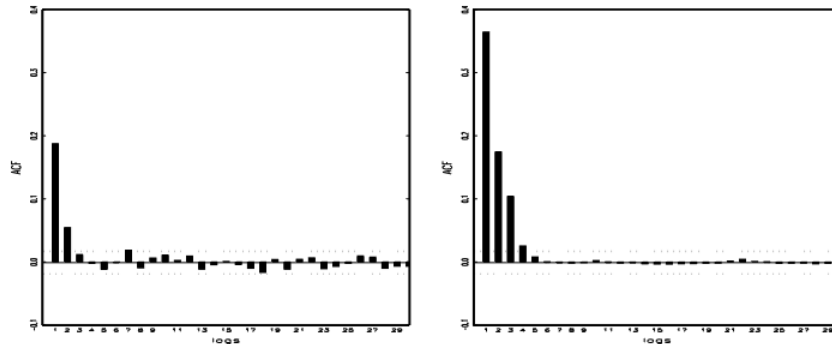
autocorrelation functions of squared time series with ARCH(1) conditional variance with \alpha = 0.2 (left panel) and \alpha = 0.7 (right panel)
