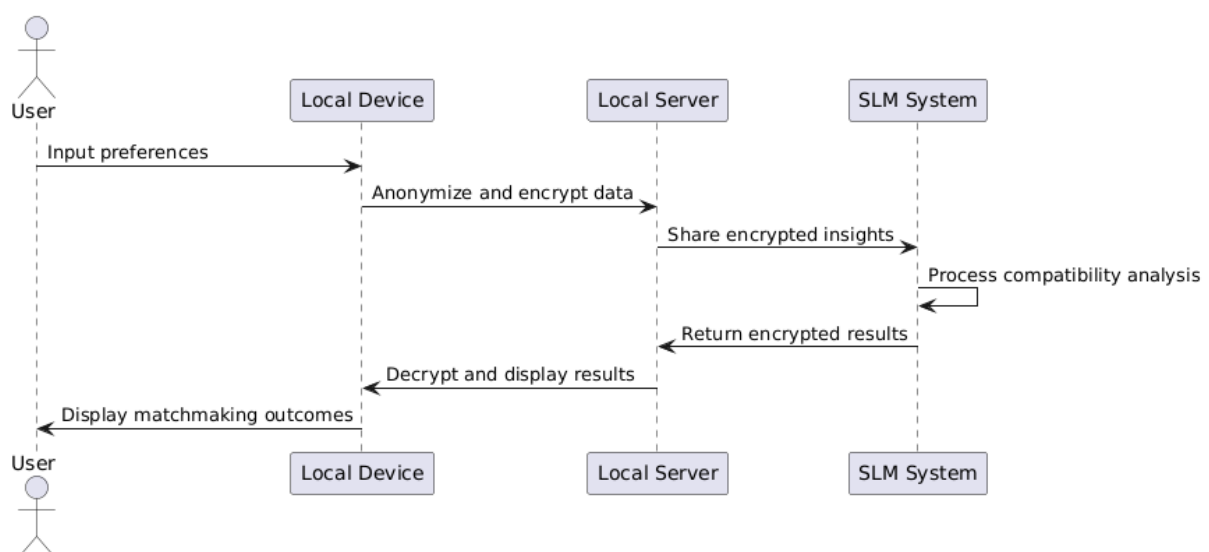
Figure 10: Sequence Diagram depicting decentralized data sharing between devices and SLM.
