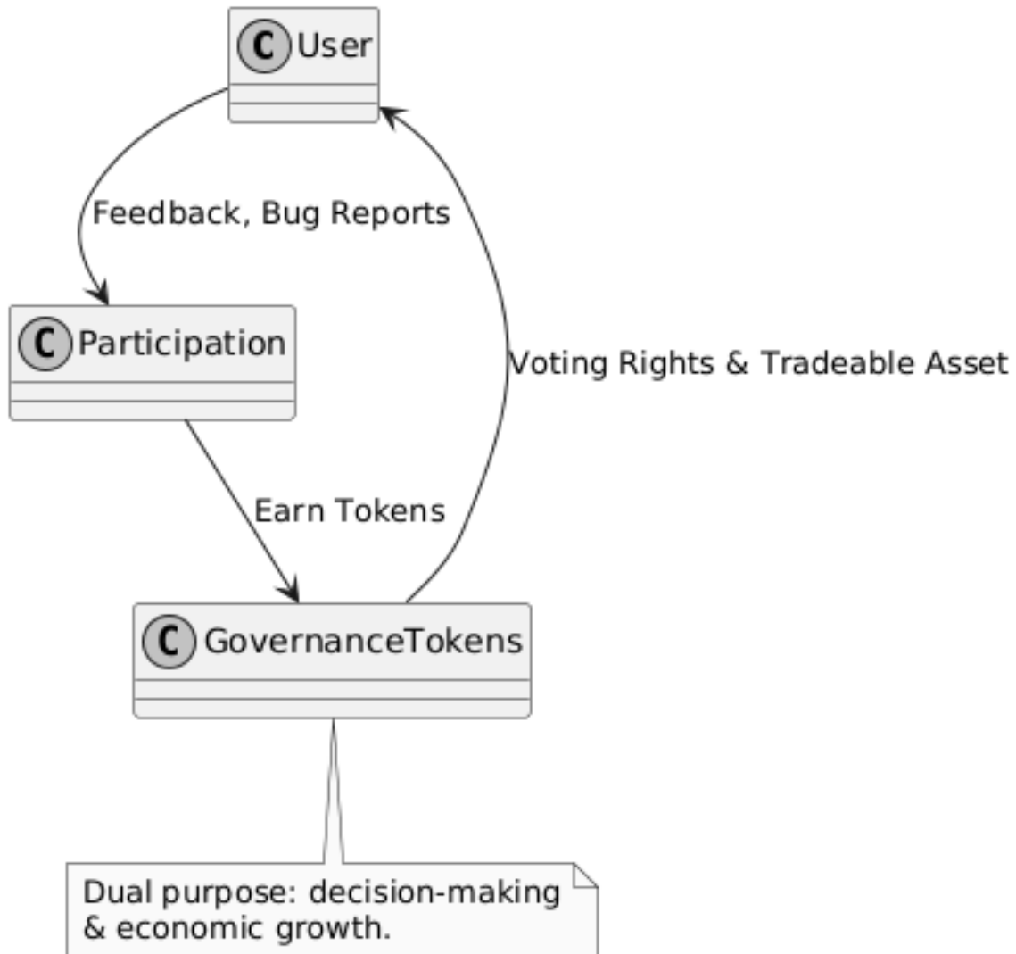
Figure 17: Incentivized Participation
